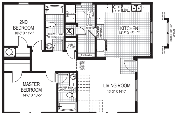
1127 Sq. Ft. 29'8" x 36'0"/40'0"
