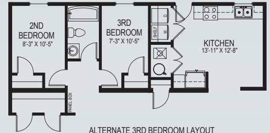
ALTERNATE 3RD BEDROOM LAYOUT
