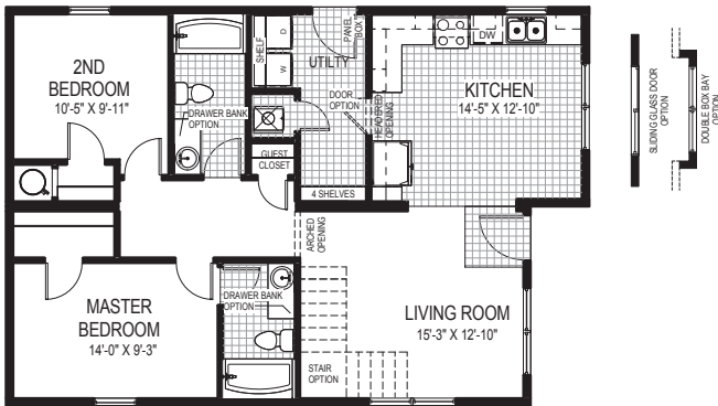
1034 Sq. Ft. 27'4" x 36'0"/40'0"
